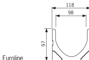
Euroline
