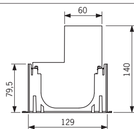
Hexa Designline
