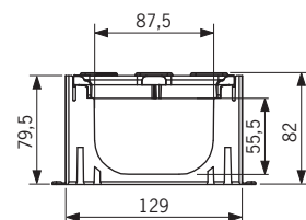
HexDrain Garagepack
