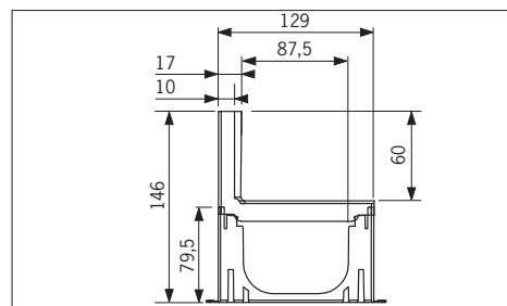
Hexa Drain Slotline
